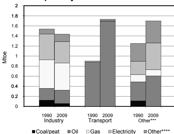
Figure 4. Breakdown of sectorial final consumption by source in 1990 and 2009**
